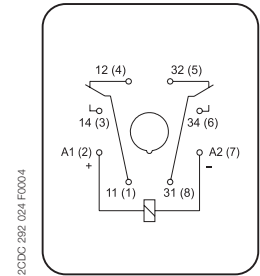
CR-U with 2 c/o contacts
