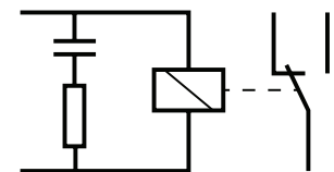
Leakage current protection
